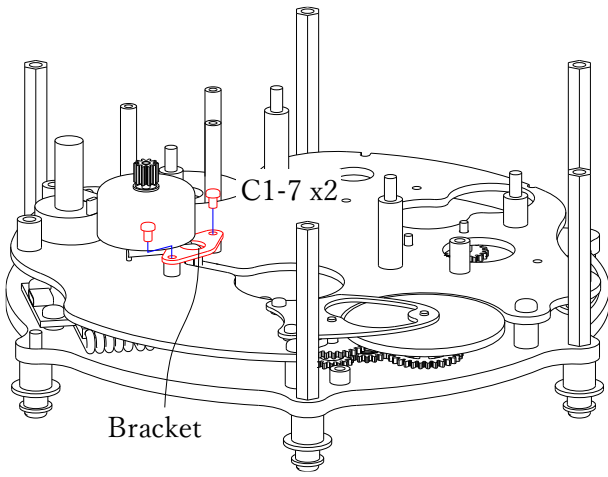
5. Pull out Bracket (D6) above MA1 and screw.
