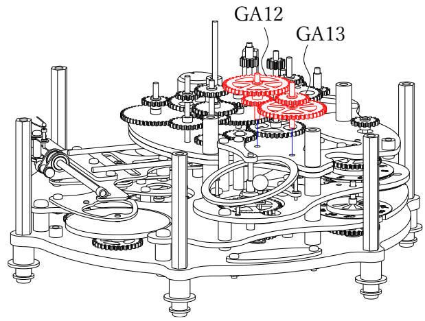
49. Attach the Saturn drive system gears GA12 and GA13.
