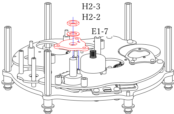
7. Tighten H2-3 using pliers. Be careful not to scratch E1-7 with the pliers.
