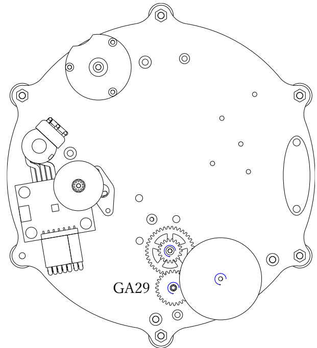
48. Rotate GA29 counterclockwise to ensure all gears rotate freely without obstruction.
