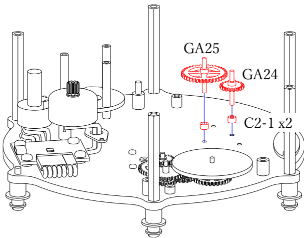
49. As in Step 46, pass GA24 and GA25 through C2-1 into the hole.
