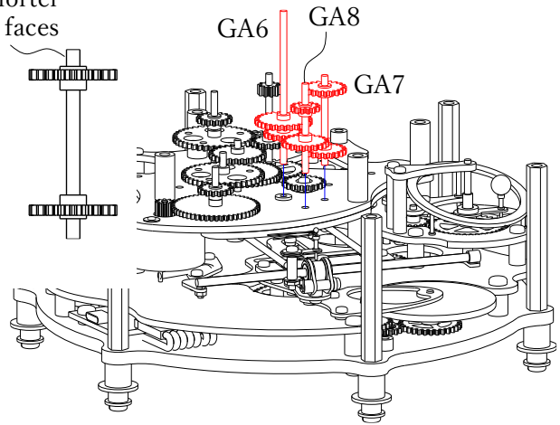
45. Attach the Mercury drive gear GA6, the gear GA7 that drives the Moon (see figure above), and the Venus drive gear GA8.
