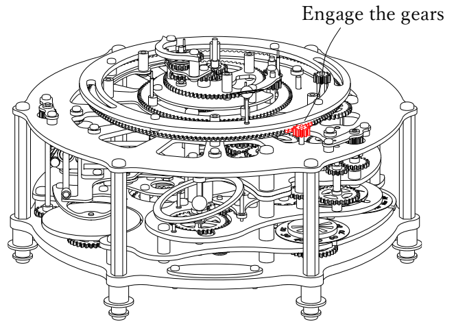
74. Engage the Saturn gear GA45 with the drive gear as shown.
