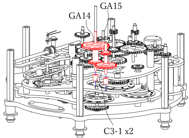
51. Attach the Saturn drive gear GA14 and the Uranus drive system gear GA15.
