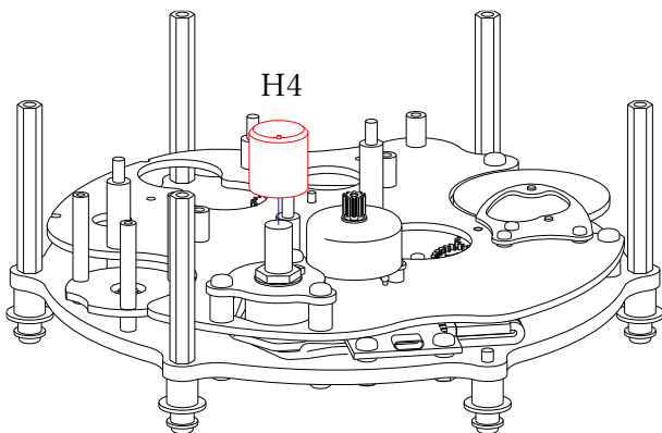
9. Turn the variable resistor fully counterclockwise, then press the knob (H4) in place in the direction shown in Step 11.
