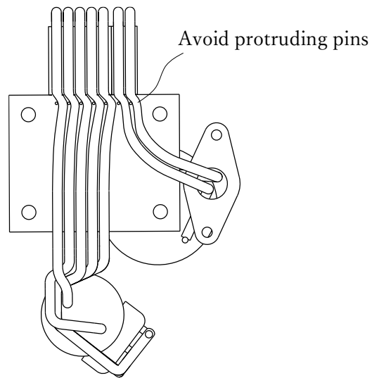
39. Bottom view
