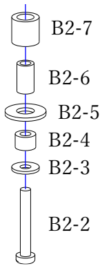
15. Make six identical units. These will serve as the legs of the product.
