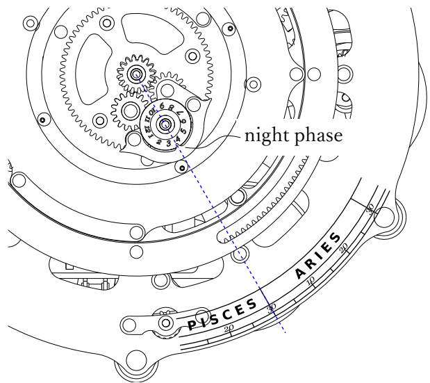
76. Connect the USB cable, turn the switch on, and rotate the Stellar Movements. As in Steps 69 and 70, align the night-phase protrusion and March 21 (vernal equinox) of the calendar with the boundary between PISCES and ARIES.
