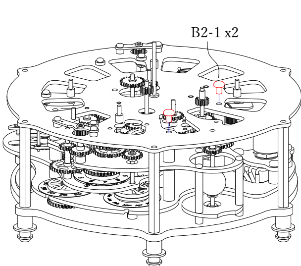
60. Lightly fasten MA4 with screws. Then rotate each gear slightly in the circumferential direction and confirm that they move freely with only the normal tooth clearance. If movement is not smooth or feels heavy, verify that no gears are riding over others and that all shafts are inserted correctly.
