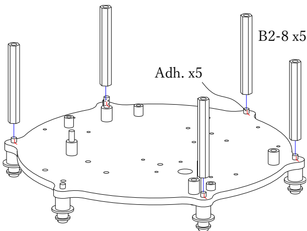
17. Apply adhesive to the base of five screws and screw in B2-8.
