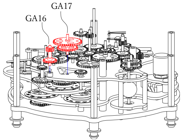
53. Attach the Uranus drive gear GA16 and the Time-scale coupling gear GA17.
