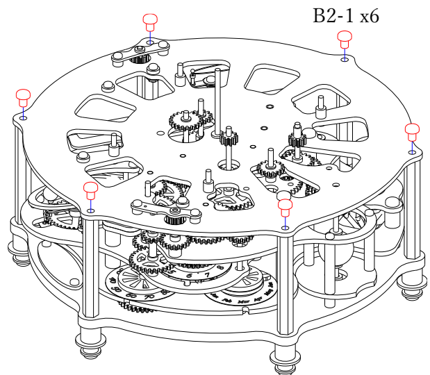
61. Fully tighten the screws from Step 60, and then firmly tighten the other six screws as well.
