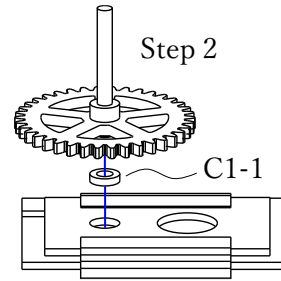
3. Use C1-1 temporarily as a jig. Return it to it after use.
