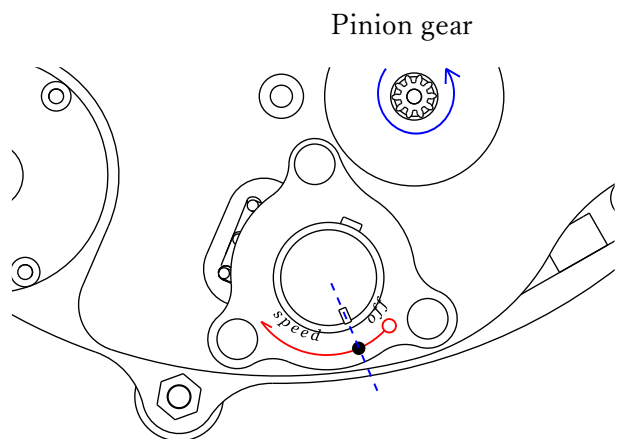
10. Align the notch of the knob toward the black dot in the diagram. If the inner groove of the knob and the groove of the variable resistor are not perfectly aligned, the notch and black dot may slightly deviate — this is not an issue.
