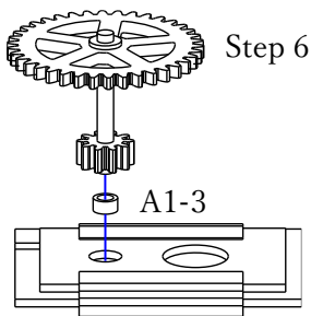
7. Use A1-3 temporarily as a jig. Return it after use.
