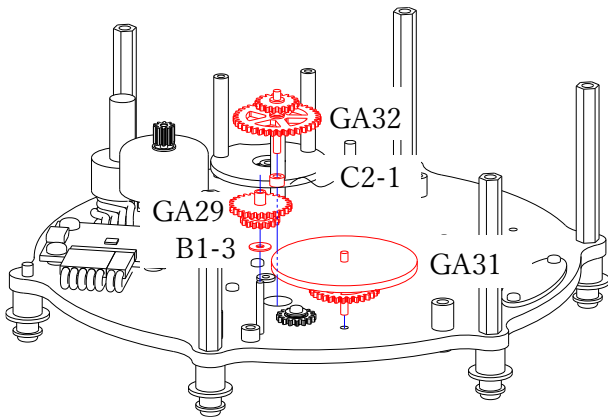
47. Pass GA32, GA29, and GA31 through the holes and shafts sequentially. Make sure not to forget C2-1 or B1-3.
