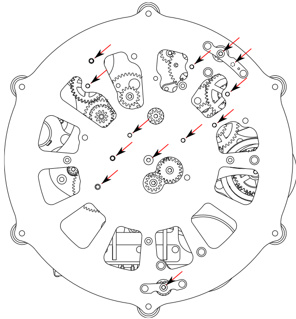
58. Top view (arrows indicate the MA4 hole positions where the shafts are inserted)
